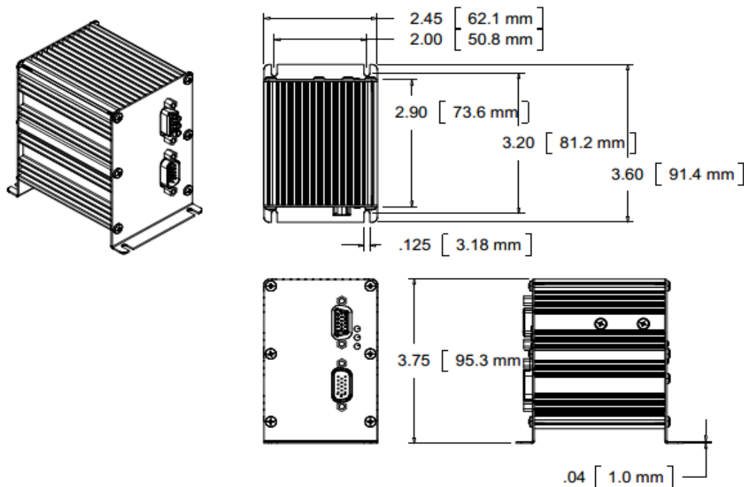
QCI-S2-IG Mechanical
