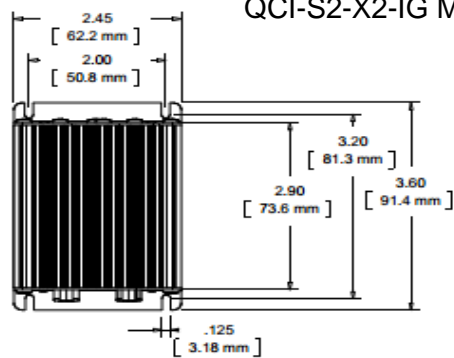
QCI-S2-X2-IG Mechanical
