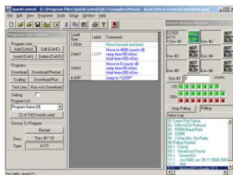
QuickControl® Integrated Development Environment
