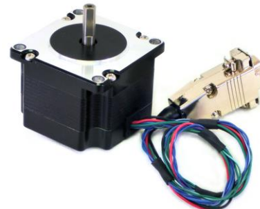
NEMA 17 and 34 Mosolver Mosolvers=Motor+Resolver
