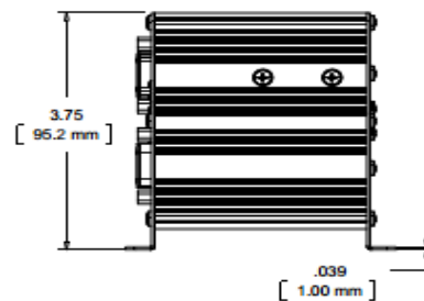
QCI-S2-IG-01 Mechanical
