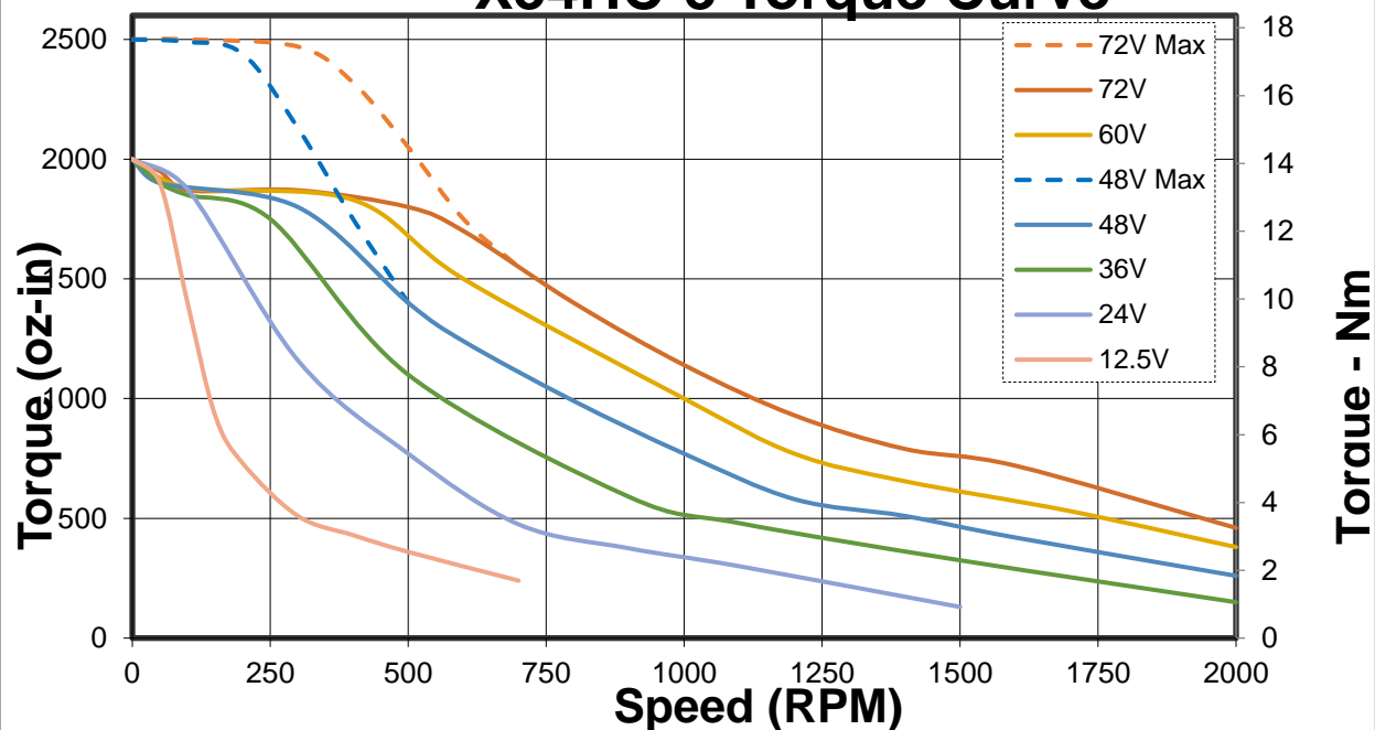
X34HC-3 Torque Curve
