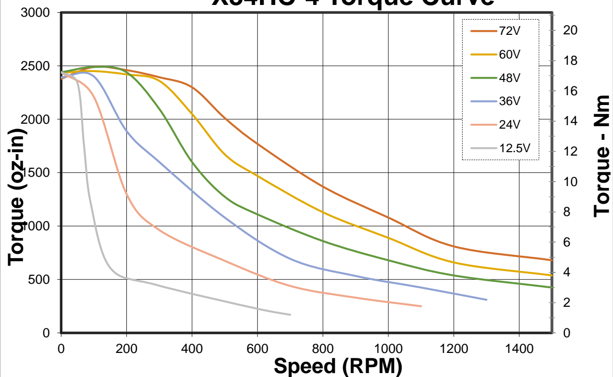
X34HC-4 Torque Curve
