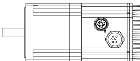
QCI-X34C-x Mechanical
