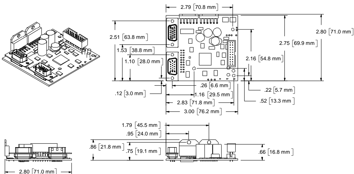
QCI-D2IG-01 Dimensions
