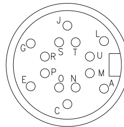
EXPOSED FRONT VIEW OF MOTOR CONNECTOR
